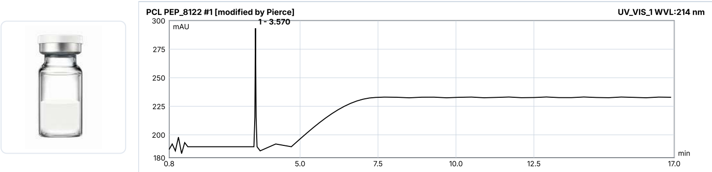
HPLC Chromatogram (Retention Time: 3.57 min)
