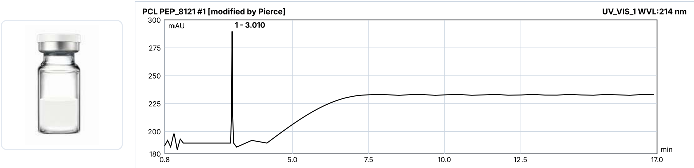
HPLC Chromatogram (Retention Time: 3.01 min)
