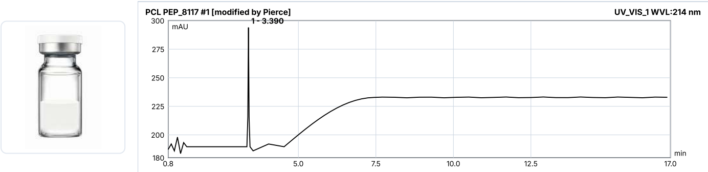
HPLC Chromatogram (Retention Time: 3.39 min)
