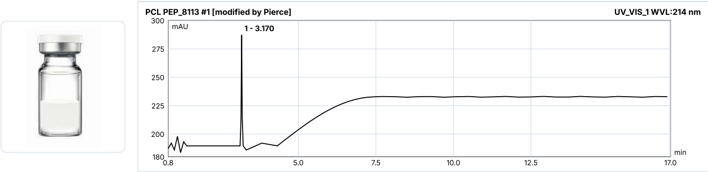
HPLC Chromatogram (Retention Time: 3.17 min)
