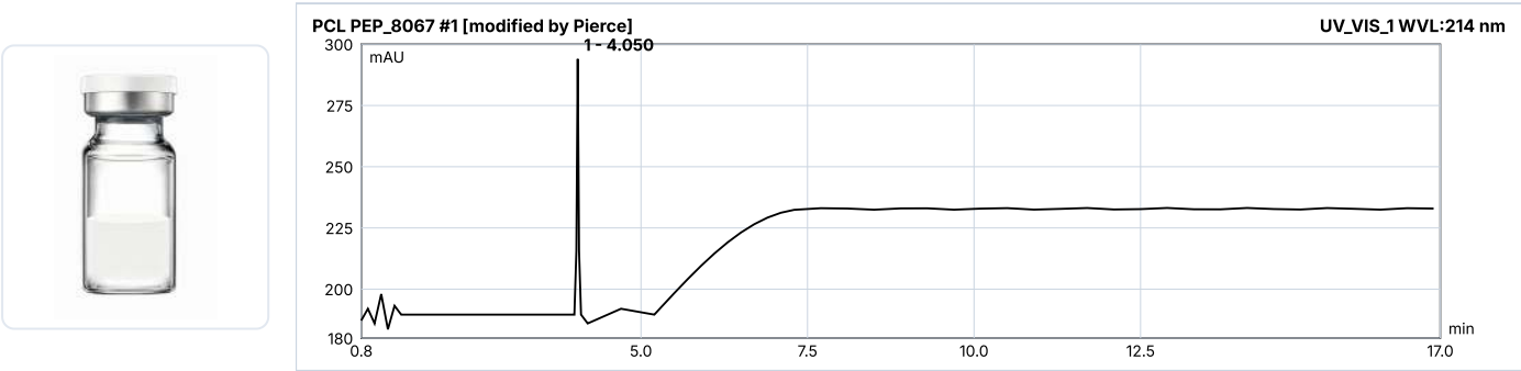
HPLC Chromatogram (Retention Time: 4.05 min)
