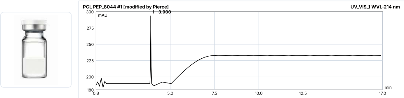
HPLC Chromatogram (Retention Time: 3.9 min)
