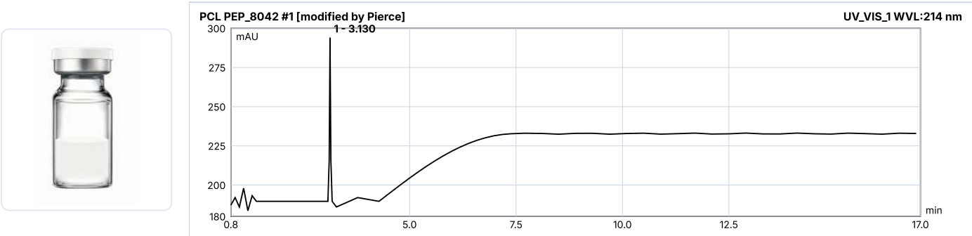
HPLC Chromatogram (Retention Time: 3.13 min)
