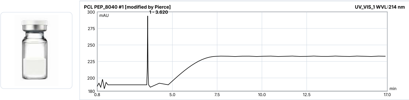
HPLC Chromatogram (Retention Time: 3.62 min)
