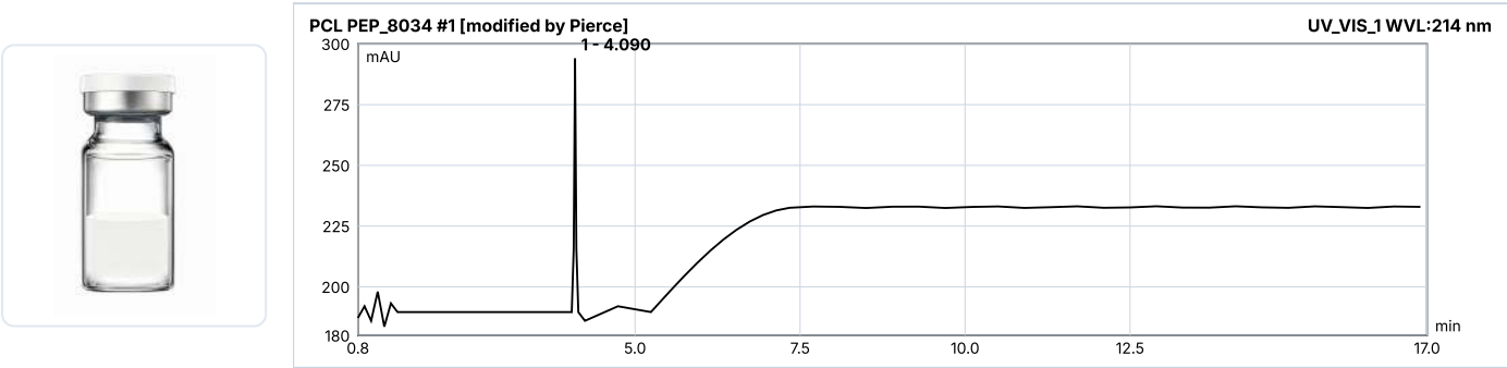
HPLC Chromatogram (Retention Time: 4.09 min)
