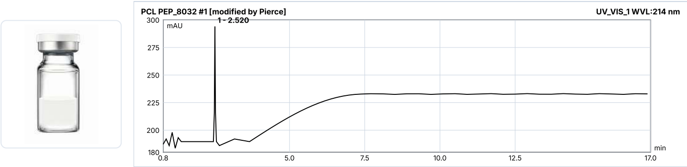
HPLC Chromatogram (Retention Time: 2.52 min)
