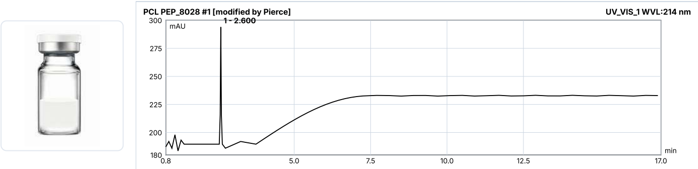
HPLC Chromatogram (Retention Time: 2.6 min)
